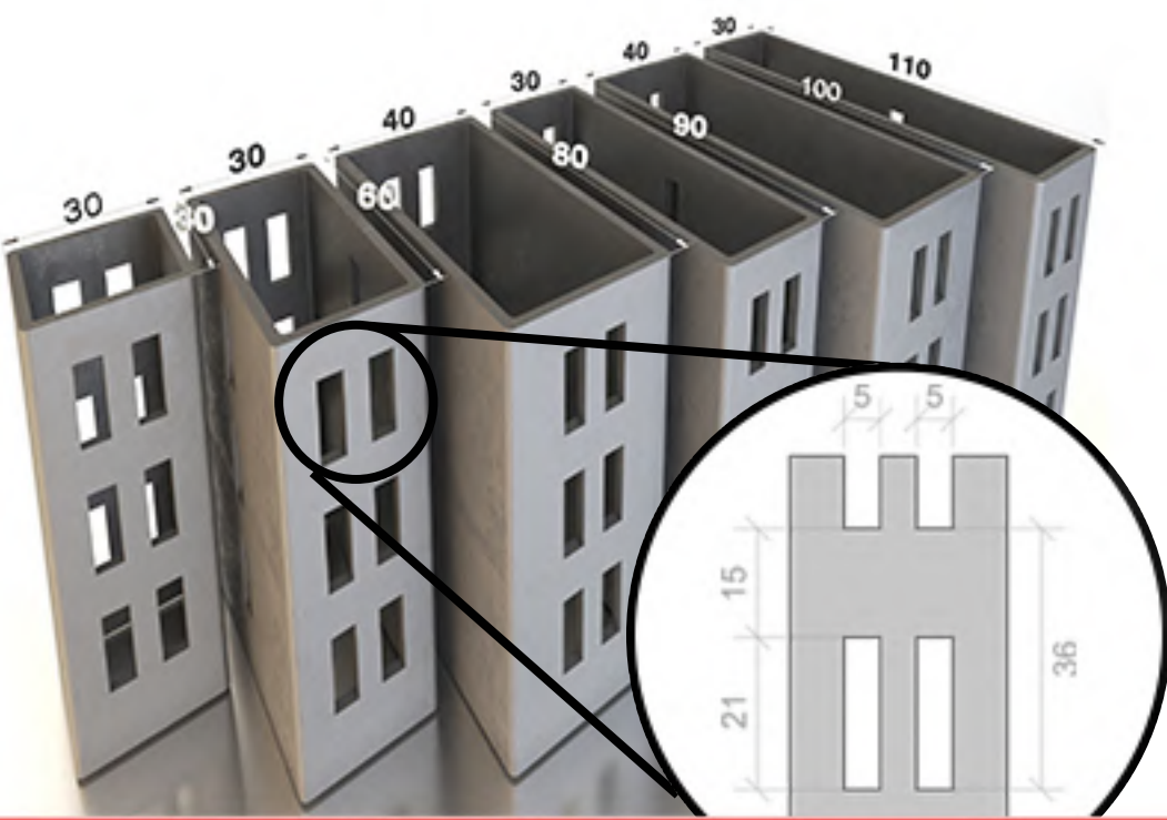
Shelf Upright Sizes Minimum 30mm to maximum 110mm
