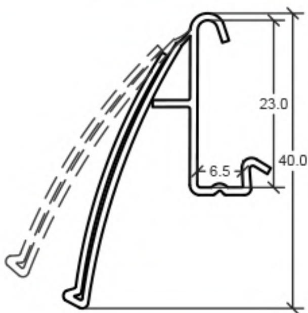
Flippy arch J-series
