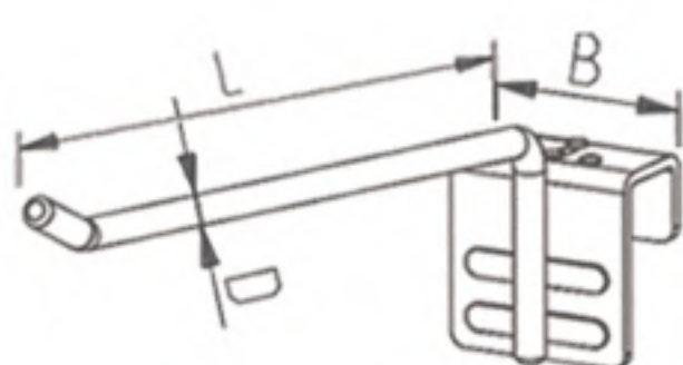
Single prong hook
