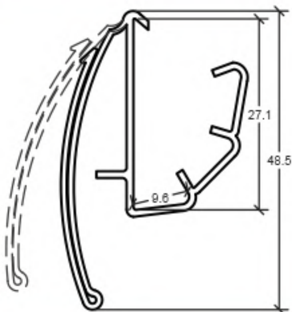
Fixed arched with edge
